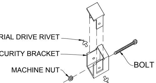
UNIVERSAL BRACKET DETAIL 1"=1'-0"
