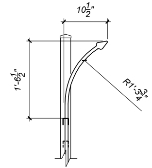
CURVED TOP PICKET DETAIL A 1/2"=1'-0"
