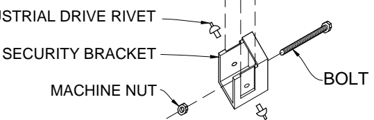
INDUSTRIAL DRIVE RIVET SECURITY BRACKET MACHINE NUT BOLT NOTE: MINIMUM SHEER STRENGTH 3,000 LBS AND HOLDING POWER OF 2,200 LBS. GUARDSMAN SECURITY BRACKET DETAIL 1"=1'-0"
