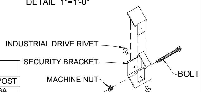
NOTE: MINIMUM SHEER STRENGTH 3,000 LBS AND HOLDING POWER OF 2,200 LBS. GUARDSMAN SECURITY BRACKET DETAIL 1"=1'-0"
