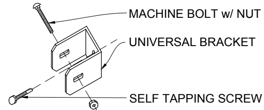
UNIVERSAL BRACKET DETAIL 1"=1'-0"
