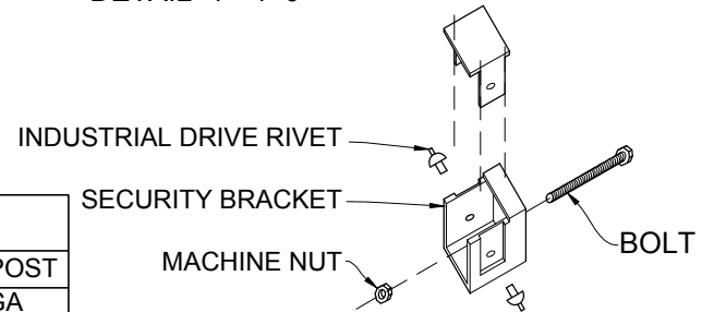
GUARDSMAN SECURITY BRACKET DETAIL 1"=1'-0"
