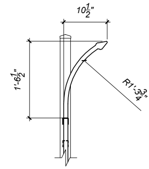
CURVED TOP PICKET DETAIL A 1/2"=1'-0"
