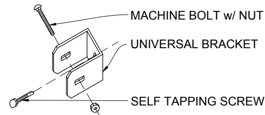
UNIVERSAL BRACKET DETAIL 1"=1'-0"
