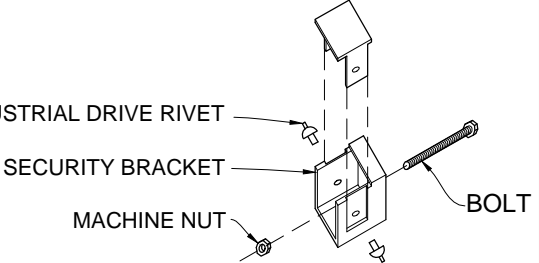
GUARDSMAN SECURITY BRACKET DETAIL 1"=1'-0"
