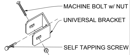
UNIVERSAL BRACKET DETAIL 1"=1'-0"
