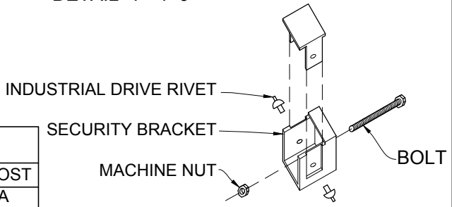
INDUSTRIAL DRIVE RIVET SECURITY BRACKET MACHINE NUT BOLT NOTE: MINIMUM SHEER STRENGTH 3,000 LBS AND HOLDING POWER OF 2,200 LBS. GUARDSMAN SECURITY BRACKET DETAIL 1"=1'-0"
