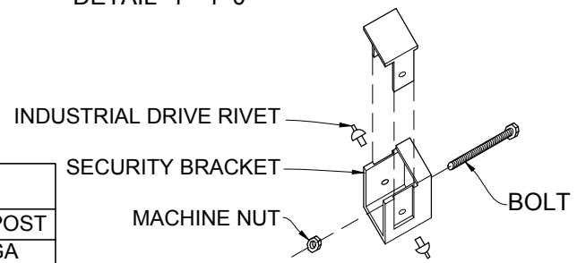
GUARDSMAN SECURITY BRACKET DETAIL 1"=1'-0" NOTE: MINIMUM SHEER STRENGTH 3,000 LBS AND HOLDING POWER OF 2,200 LBS.
