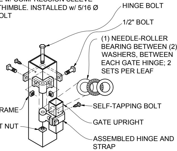
PRESSED STEEL SQUARE HINGE DETAIL - NOT TO SCALE
