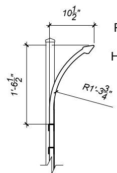
CURVED TOP PICKET DETAIL 1/2"=1'-0"
