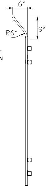
SECTION VIEW
