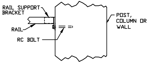
BRACKET INSTALLATION DETAIL
