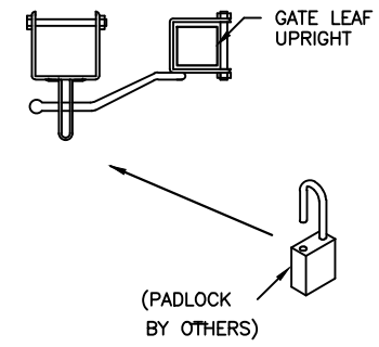
LOCKING SYSTEM
