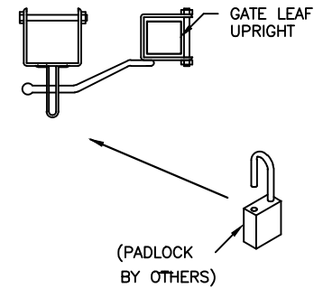
LOCKING SYSTEM
