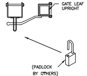
LOCKING SYSTEM
