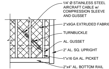
TURNBUCKLE ASSEMBLY DETAIL 1/2"=1'-0"
