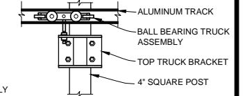
TOP TRUCK ASSEMBLY DETAIL 1/2"=1'-0"
