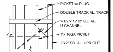
RAIL DETAIL 1/2"=1'-0"
