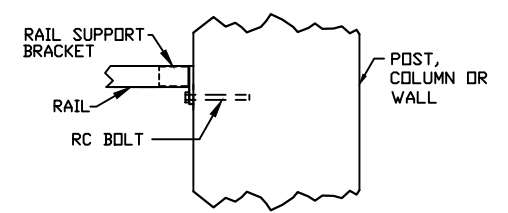
BRACKET INSTALLATION DETAIL
