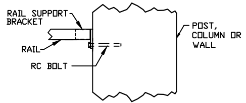
BRACKET INSTALLATION DETAIL
