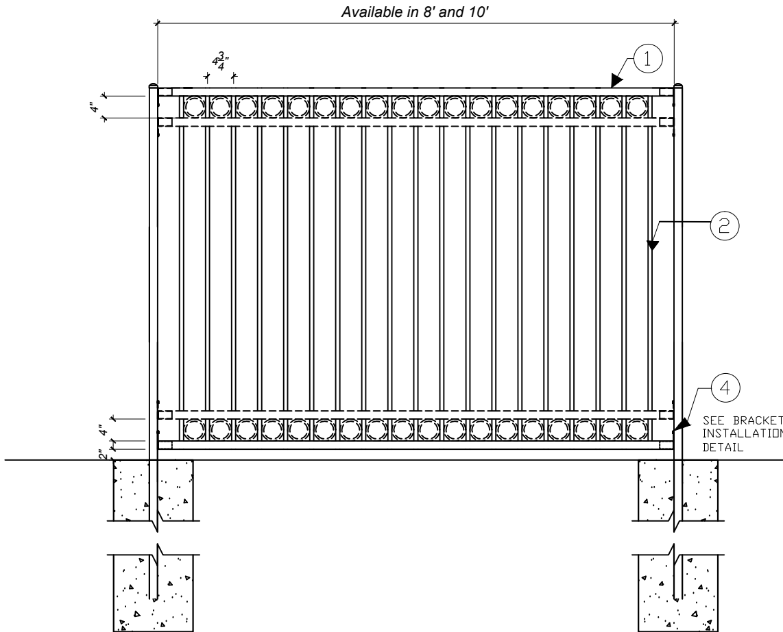
SECTION VIEW
