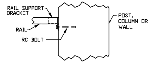
BRACKET INSTALLATION DETAIL
