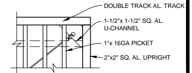
RAIL DETAIL 1/2"=1'-0"
