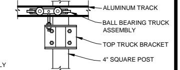
TOP TRUCK ASSEMBLY DETAIL 1/2"=1'-0"
