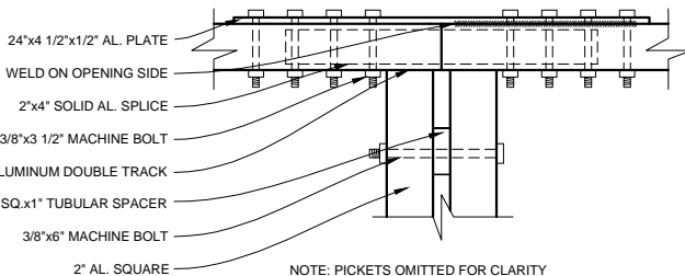
NOTE: PICKETS OMITTED FOR CLARITY TRACK HORIZONTAL SPLICE DETAIL 1"=1'-0"
