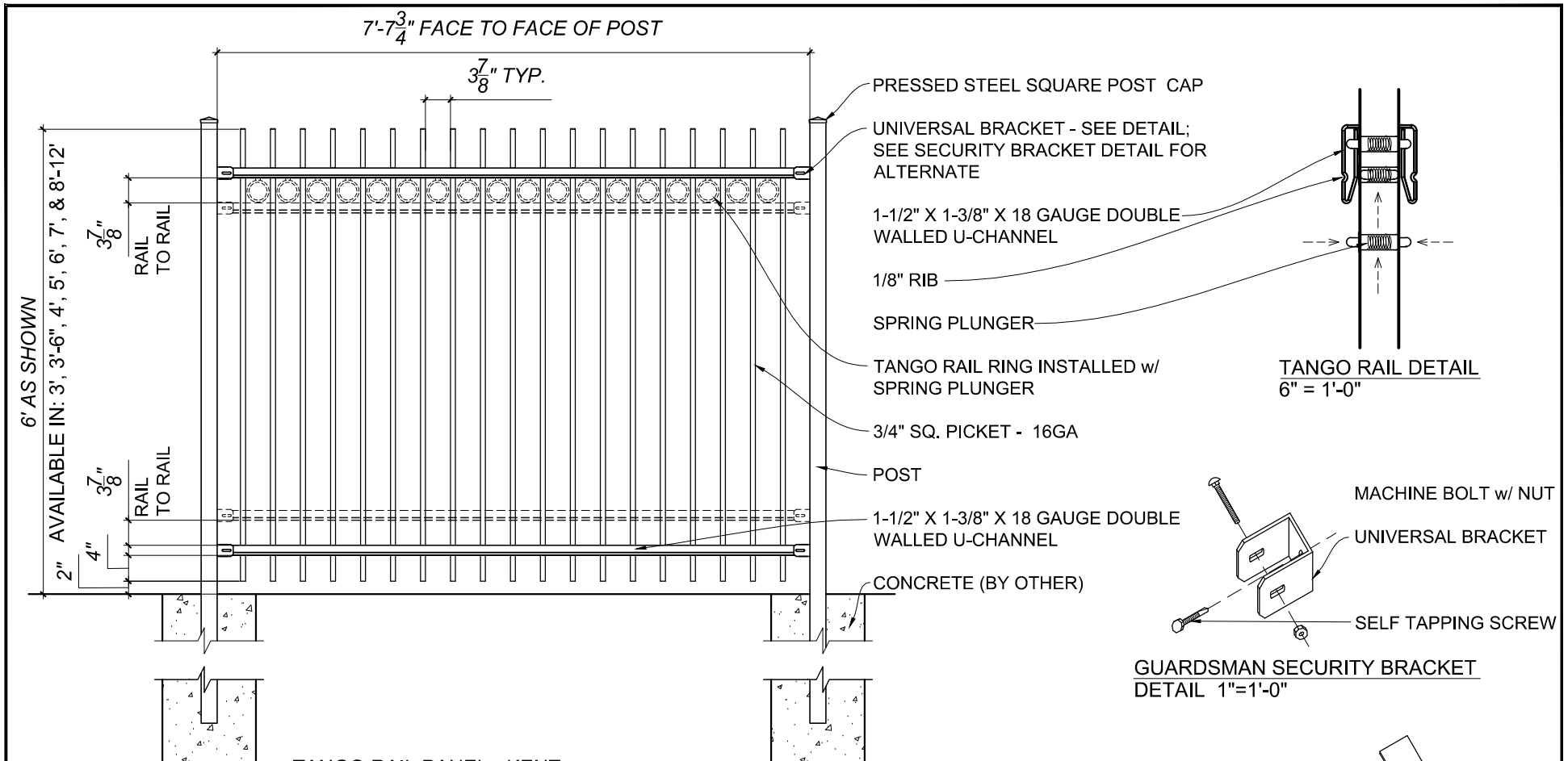
TANGO RAIL PANEL - KENT ELEVATION - OUTSIDE LOOKING IN 1/2"=1'-0"
