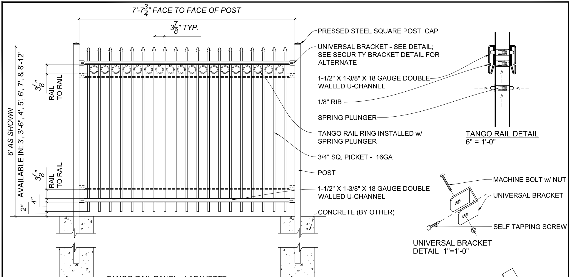
TANGO RAIL PANEL - LAFAYETTE ELEVATION - OUTSIDE LOOKING IN 1/2"=1'-0"
