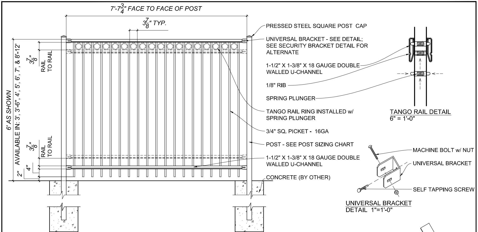
TANGO RAIL PANEL - MONROE ELEVATION - OUTSIDE LOOKING IN 1/2" = 1'-0"
