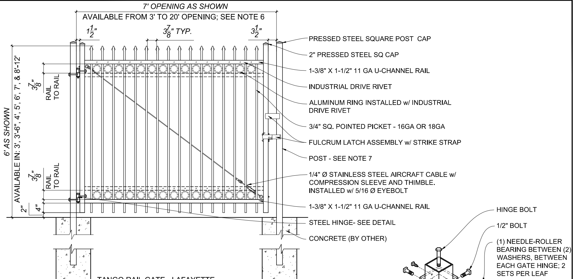
TANGO RAIL GATE - LAFAYETTE ELEVATION - OUTSIDE LOOKING IN 1/2"=1'-0"
