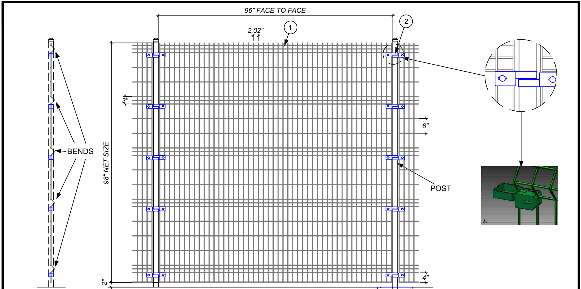
SECTION VIEW
