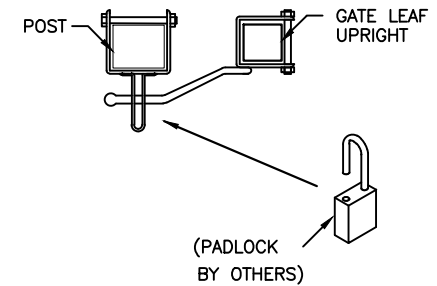
DETAIL A: LOCKING SYSTEM
