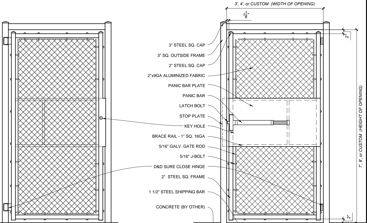
TUF GUARD GATE ELEV. OUTSIDE LOOKING IN 1/2"=1'-0"
