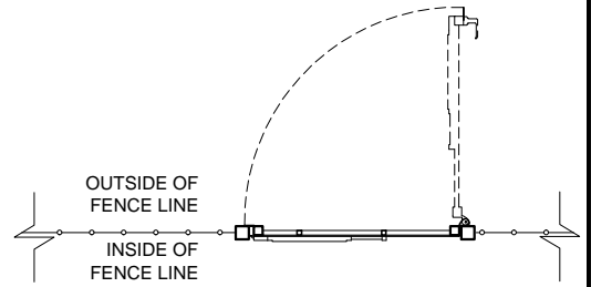
TUF GUARD GATE PLAN 1/4"=1'-0"
