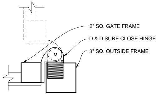
D & D SURE CLOSE HINGE DETAIL - 2"=1'-0"
