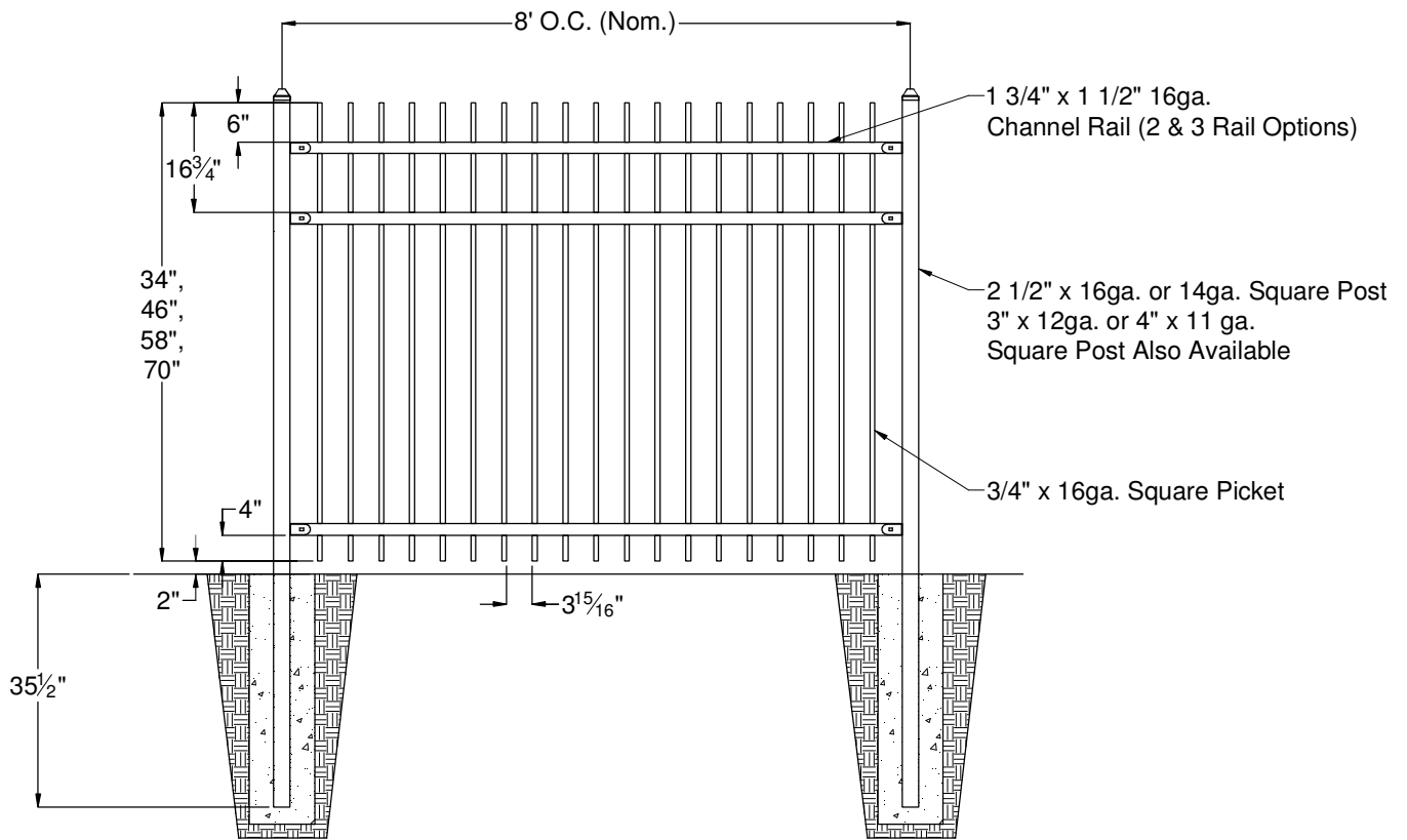
Titan Commercial Fence Panel Elevation (Typ.)
