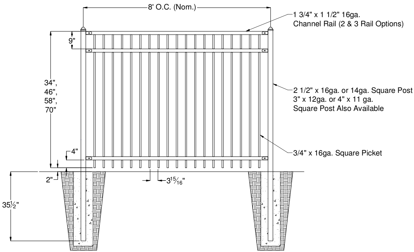
Titan Commercial Fence Panel Elevation (Typ.)
