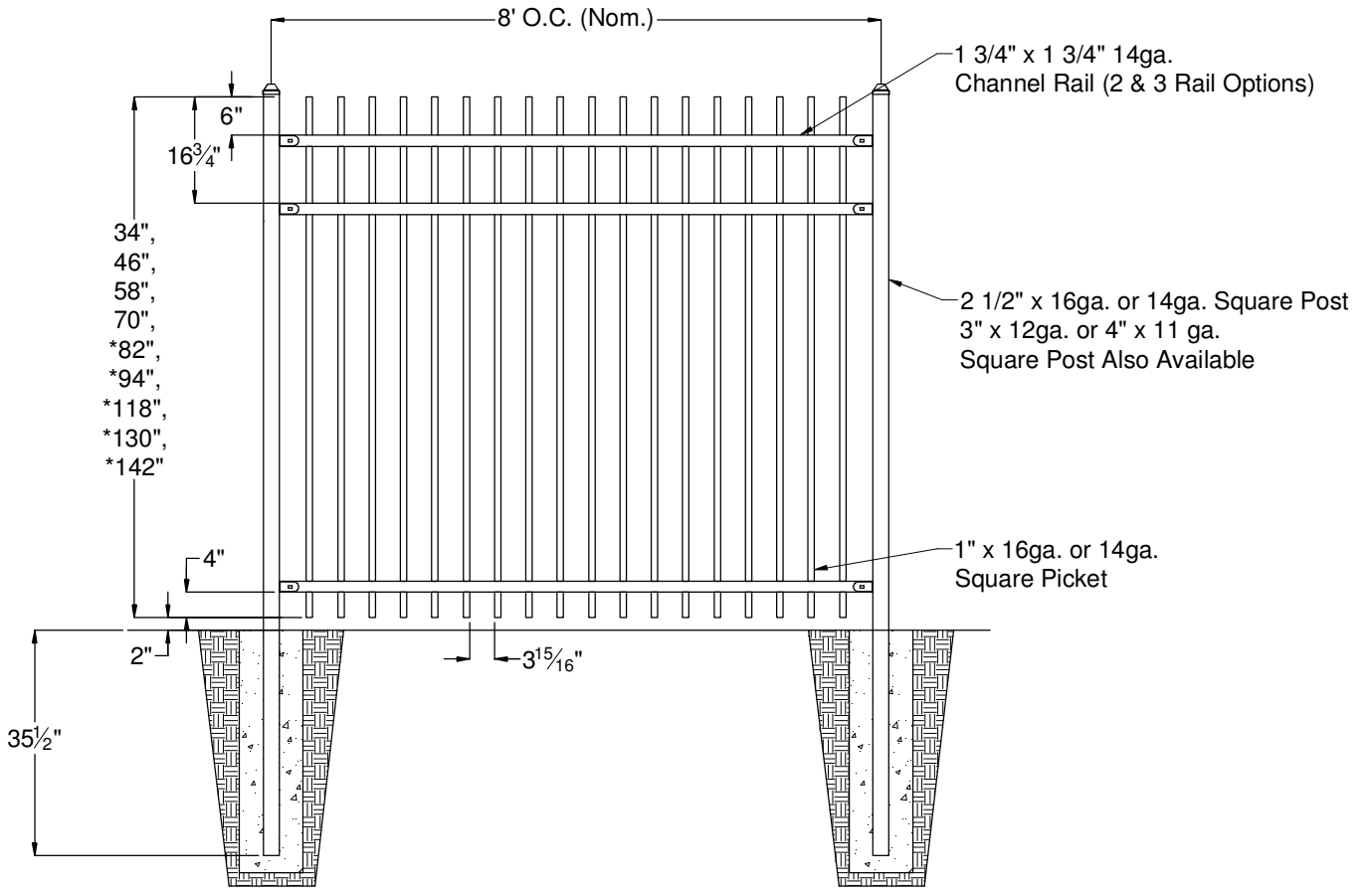
Titan Industrial Fence Panel Elevation (Typ.)
