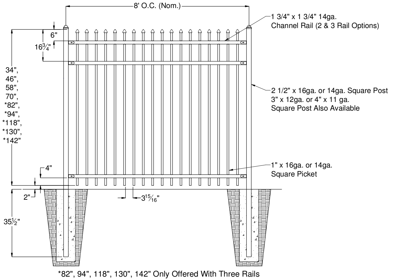
Titan Industrial Fence Panel Elevation (Typ.)
