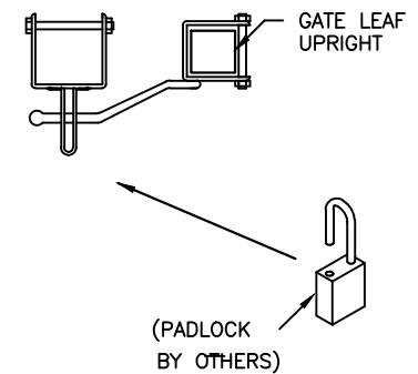
LOCKING SYSTEM
