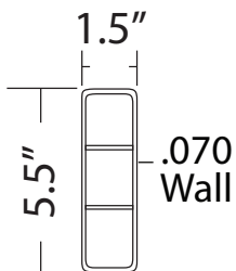
Ranch Rail Profile
